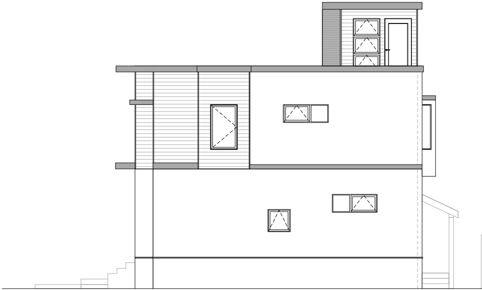
East Elevation
